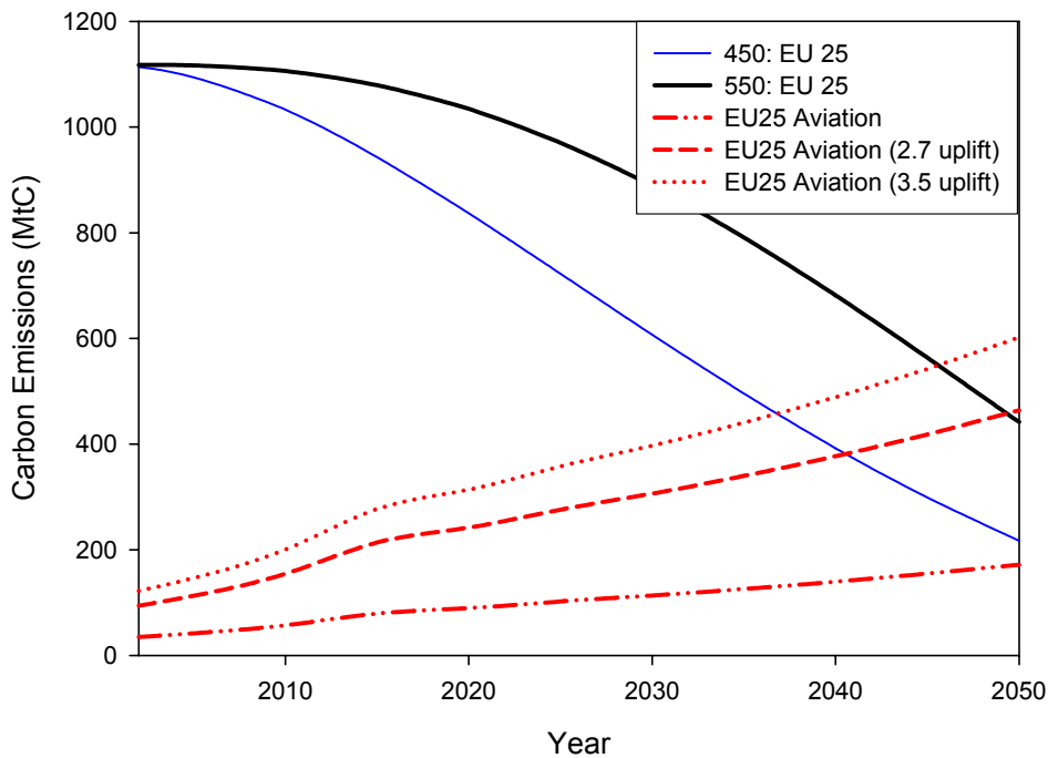
Figure 8: Contraction and convergence profiles to meet 450ppmv and 550ppmv carbon dioxide concentrations for the EU25 nations compared with their projected aviation emissions with no uplift, uplifted by 2.7 and uplifted by 3.5. Emissions profile in black thick solid line for 550ppmv, blue (thin) solid for the 450ppmv, dash-dot-dot for no uplift, short dash for an uplift of 2.7, and dotted for 3.5 uplift.
